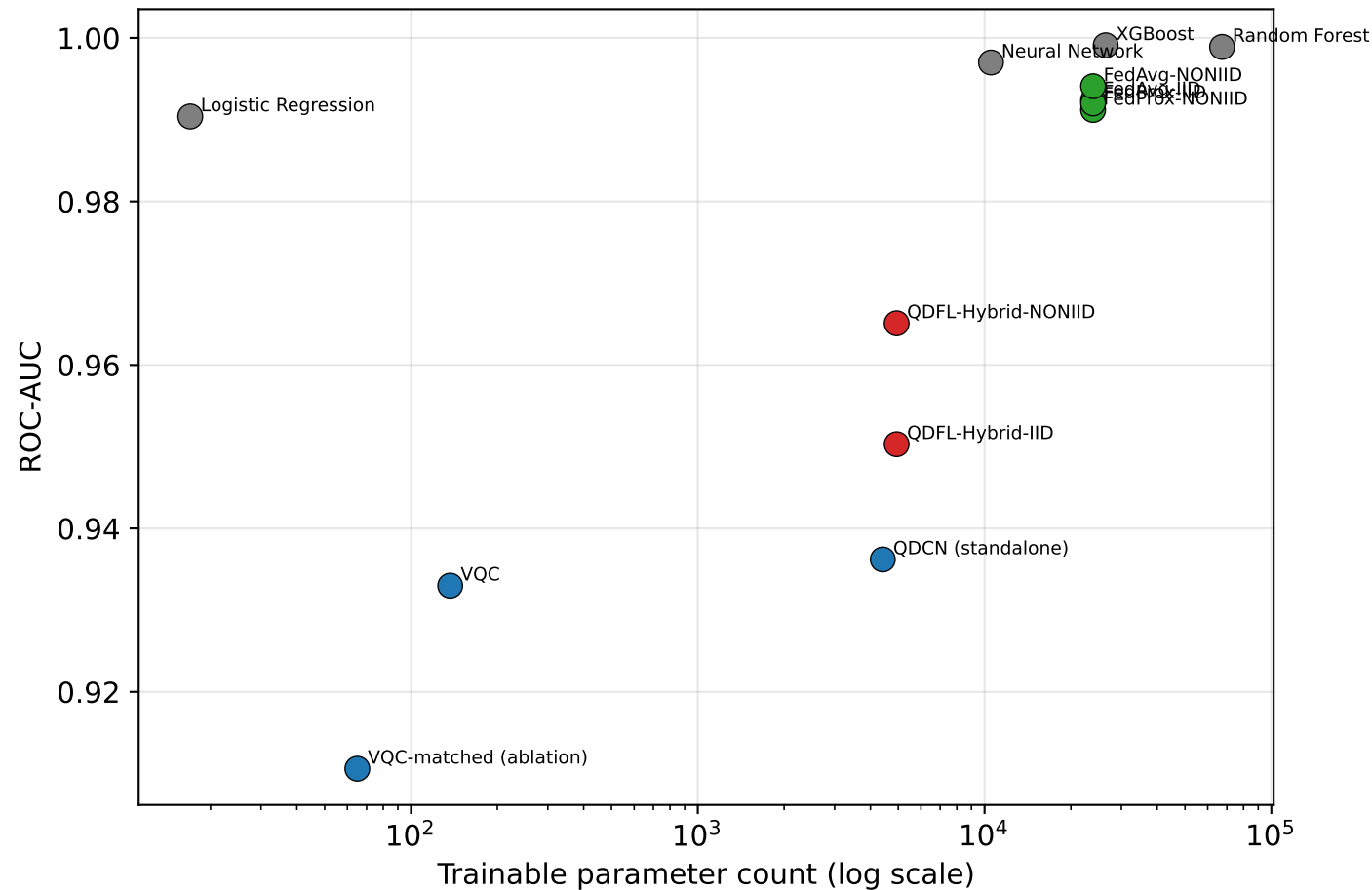
PaySim (Lopez-Rojas) Parameter-efficient Pareto (red = QDFL)
